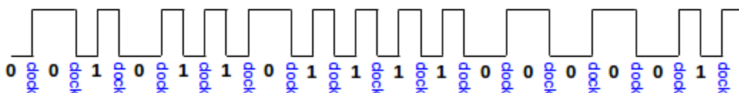
Manchester Encoding: NRZI alternating with clock transitions
