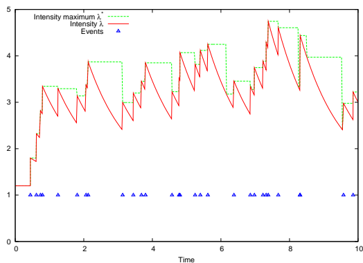
Figure: Simulation of a one-dimensional Hawkes process with parameters P = 1 , \lambda_0 = 1.2 , \alpha_1 = 0.6 , \beta_1 = 0.8 . (Zoom of the previous figure).
