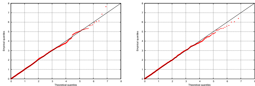
Figure: Quantile plots for one sample of simulated data of a two-dimensional Hawkes process with P = 1 and parameters given in equation (37). (Left) m = 0 . (Right) m = 1 .
