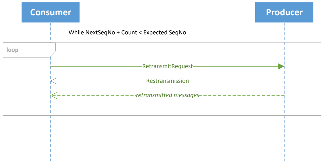
Figure 5 Retransmission Diagram
